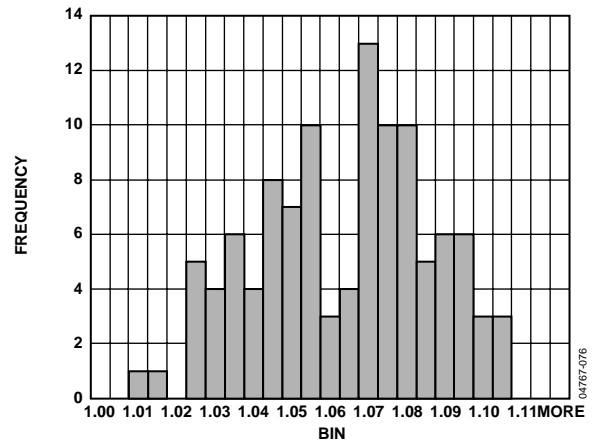
Figure 39. I_{DD} Histogram V_{DD} = 5.0V
